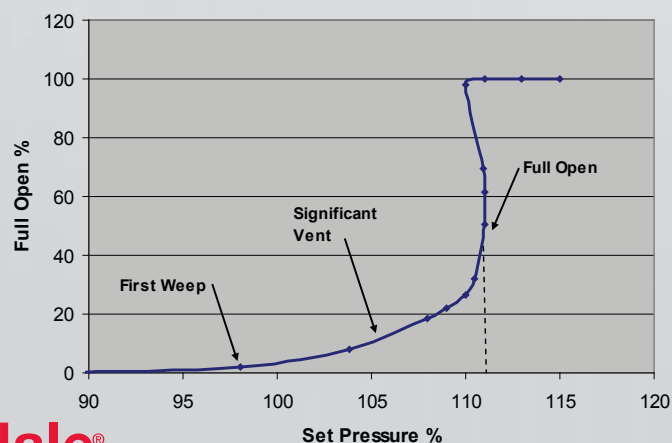
Typical 8014 Lift Characteristics
