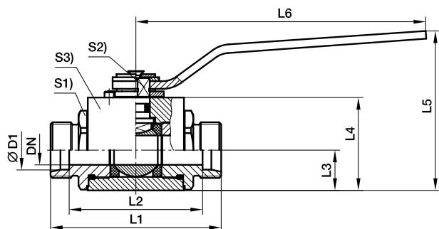
DN 4-25
