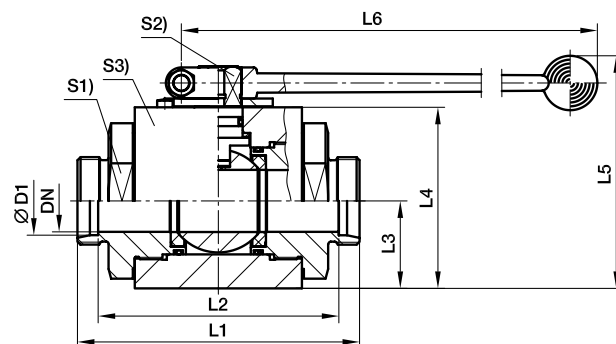
DN 32-40
