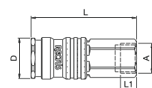
Female Thread
