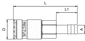
Hose Barb
