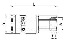
Female Thread
