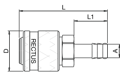
Hose Barb
