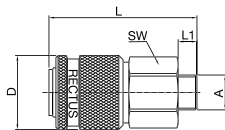
Male Thread
